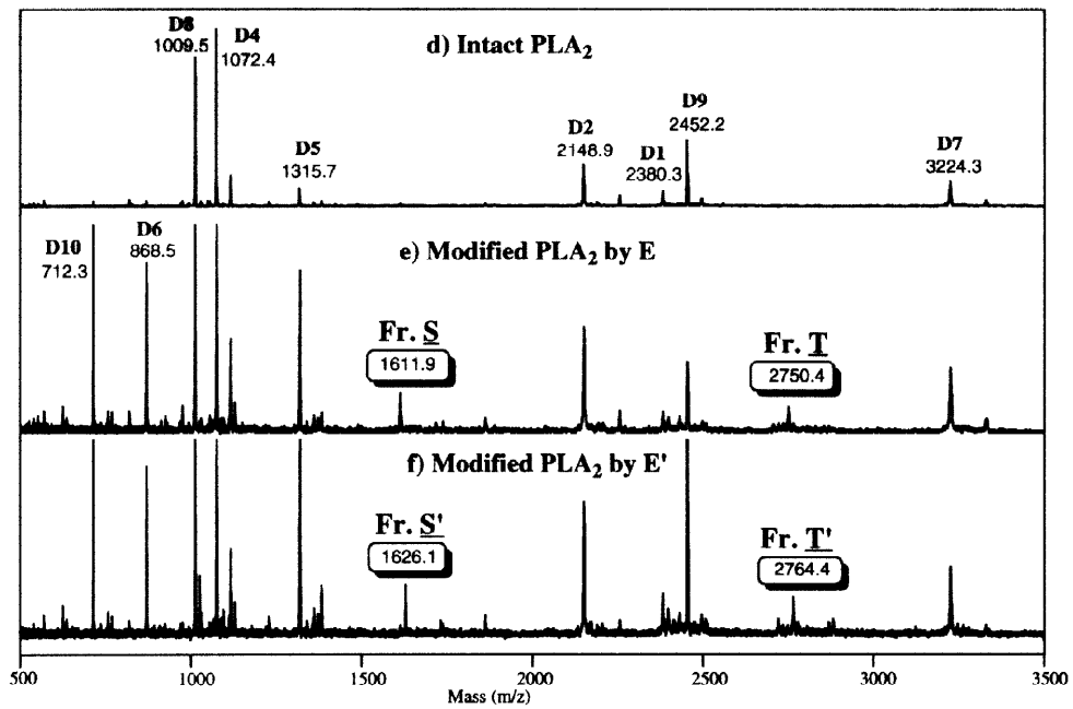
Fig. 9 MALDI-TOF mass spectra of digests by Asp-N.
