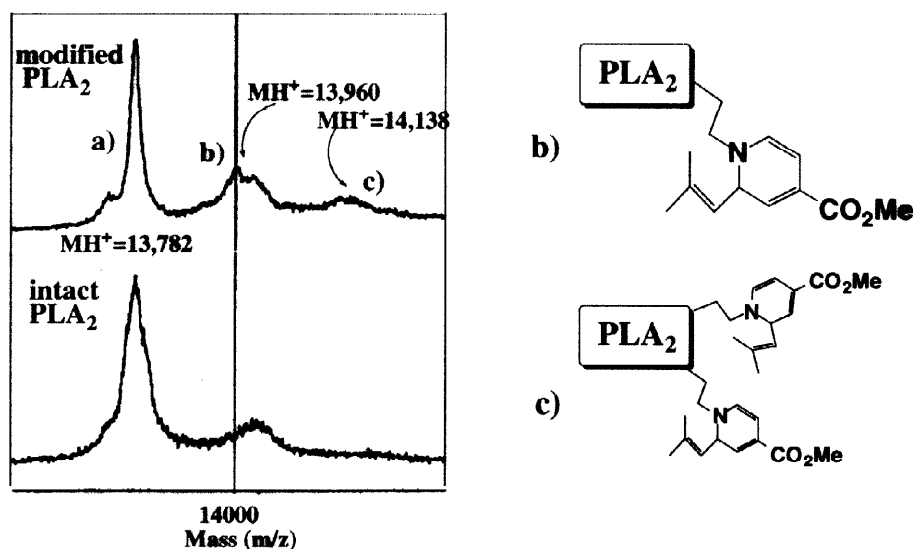
Fig. 6 MALDI - TOF MASS spectrum of the modified PLA 2 by the derivative C.
