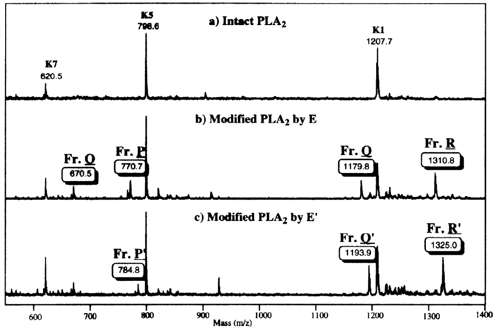
Fig. 8 MALDI-TOF mass spectra of digests by Lys-C.
