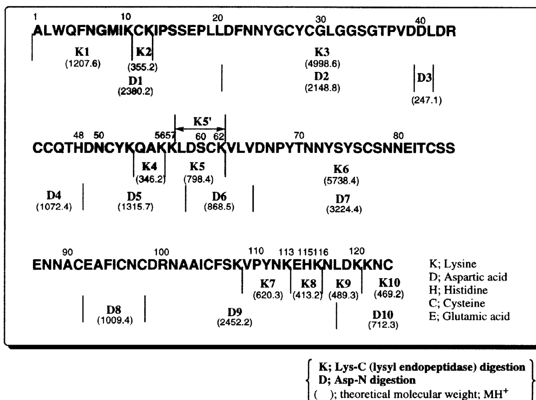
Fig. 7 Amino acid sequence of bovine pancreatic PLA 2
