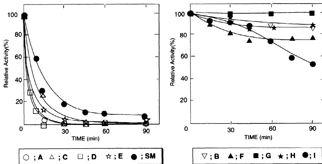
Fig. 4 Inhibition of bovine pancreatic PLA 2 by A and its derivatives.
